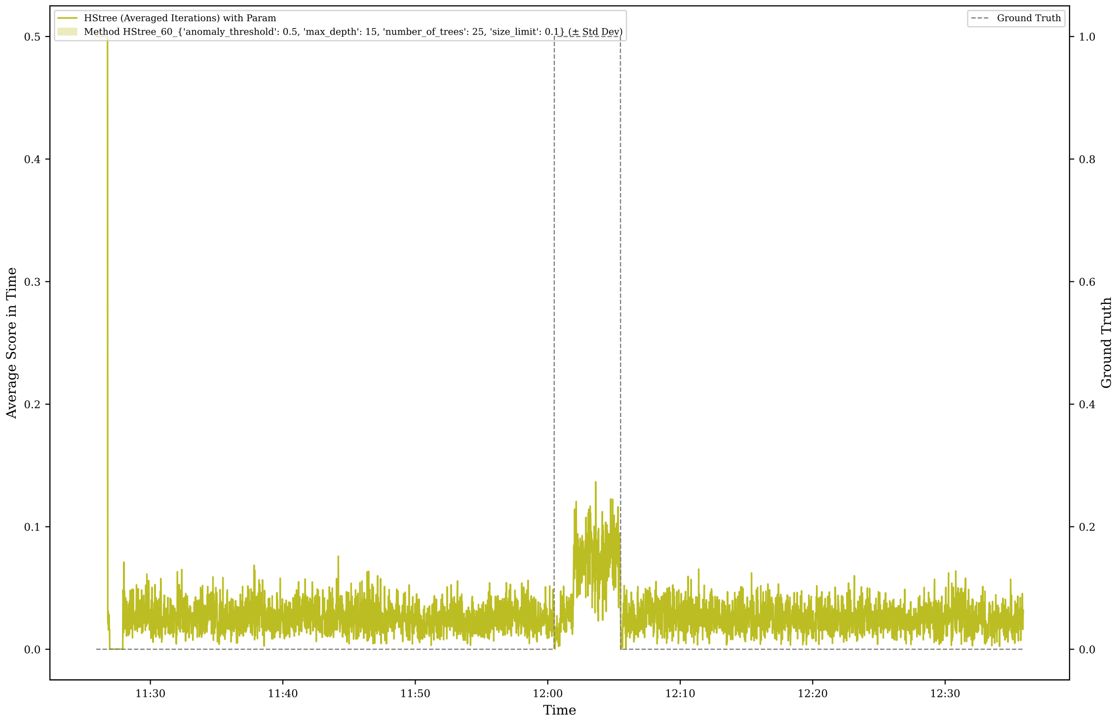
Method HStree Score for Scenario A5
